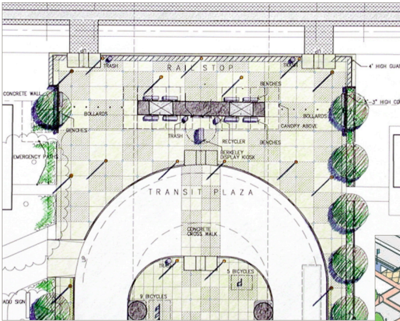
Rail Stop and Bus Turnaround Detail
